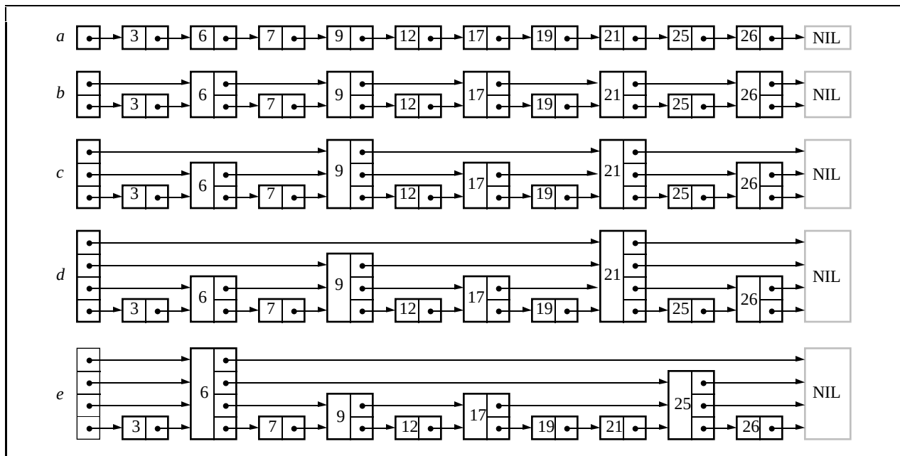
FIGURE 3 - Linked lists with additional pointers
