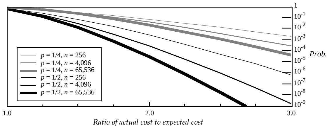
FIGURE 8 - This graph shows a plot of an upper bound on the probability of a search taking substantially longer than expected. The vertical axis shows the probability that the length of the search path for a search exceeds the average length by more than the ratio on the horizontal axis. For example, for p = 1/2 and n = 4096 , the probability that the search path will be more than three times the expected length is less than one in 200 million.
