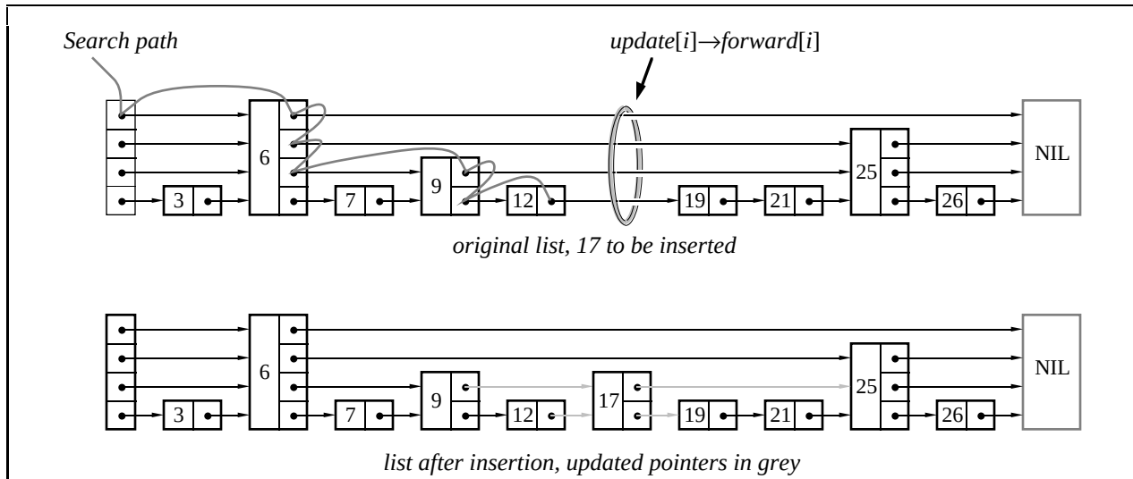
FIGURE 5 - Pictorial description of steps involved in performing an insertion
